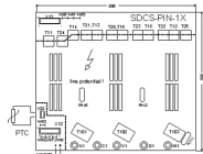
Figure 41-101: Section A-A (SDCS-PIN-1X) in back
