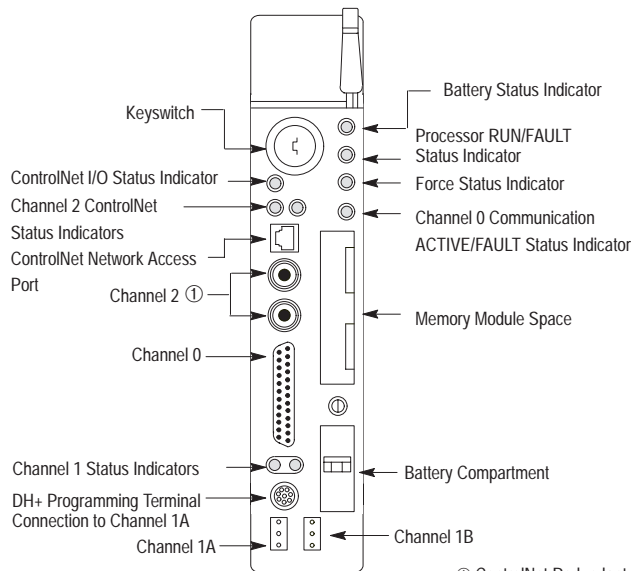
PLC-5/20C Processor
