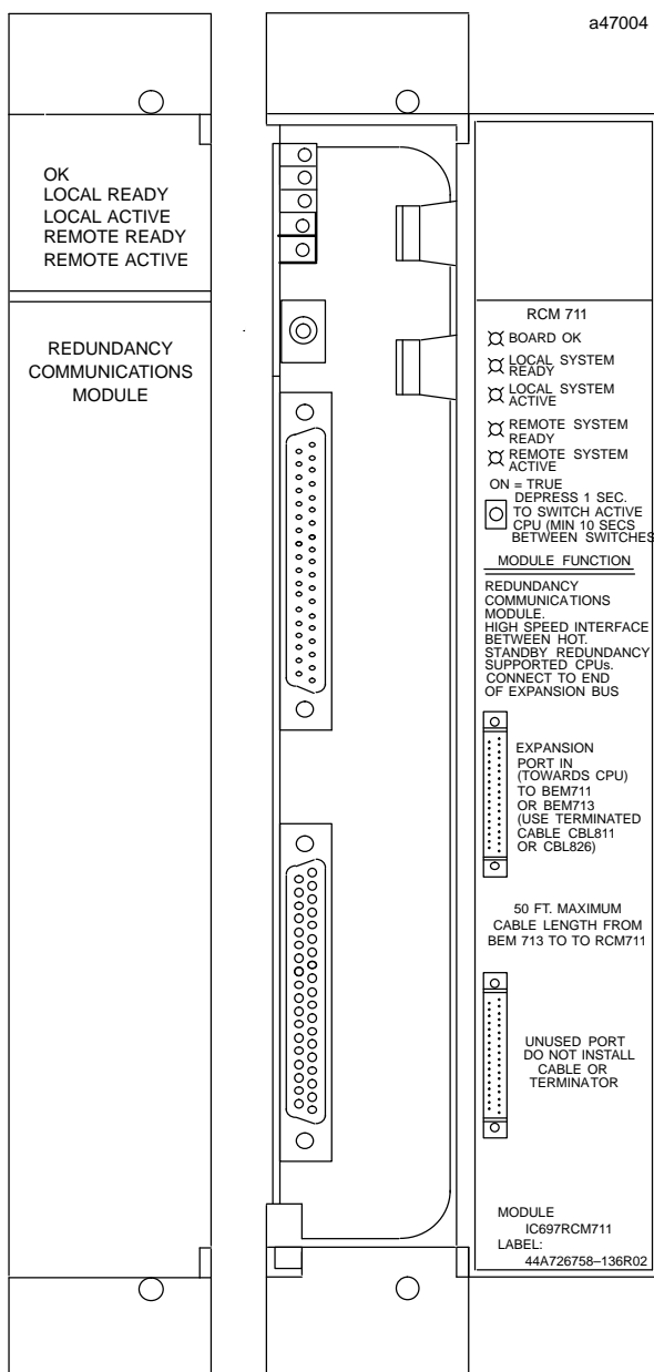
Figure 5. Redundancy Communications Module - IC697RCM711
