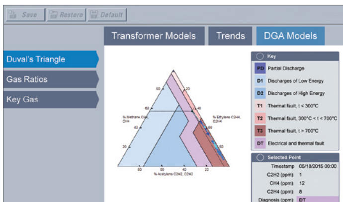
Duval Triangle DGA model
