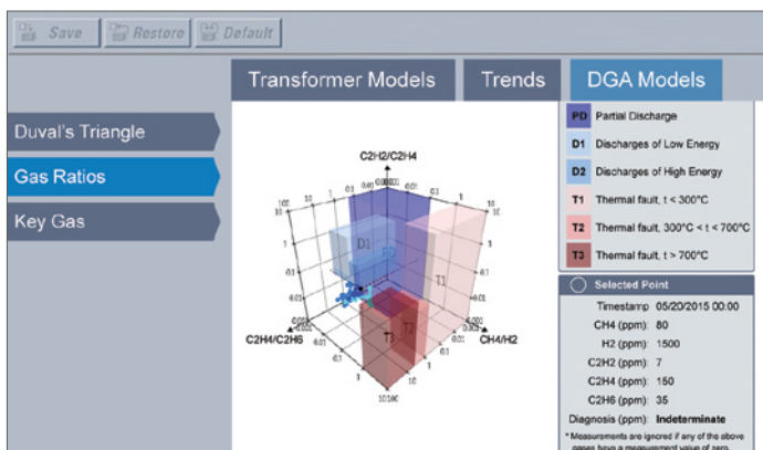
Gas Ratios DGA model
