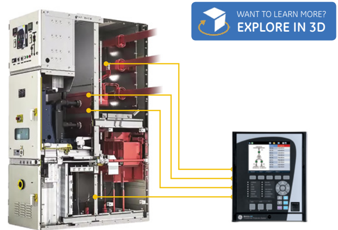
MV Switchgear or Motor Control Center
