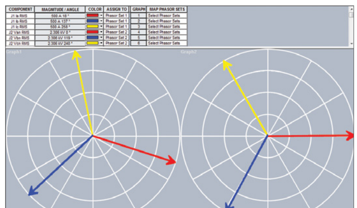
Multilin 845 Phasor viewer
