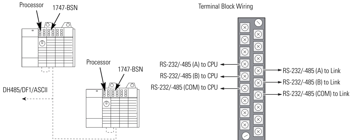
Figure 3.4 RS-232/485 System
